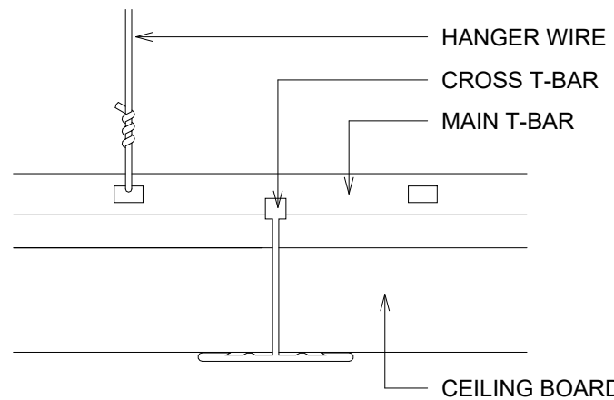
10 SECTION PERPENDICULAR TO CROSS T-BAR 1 : 100
