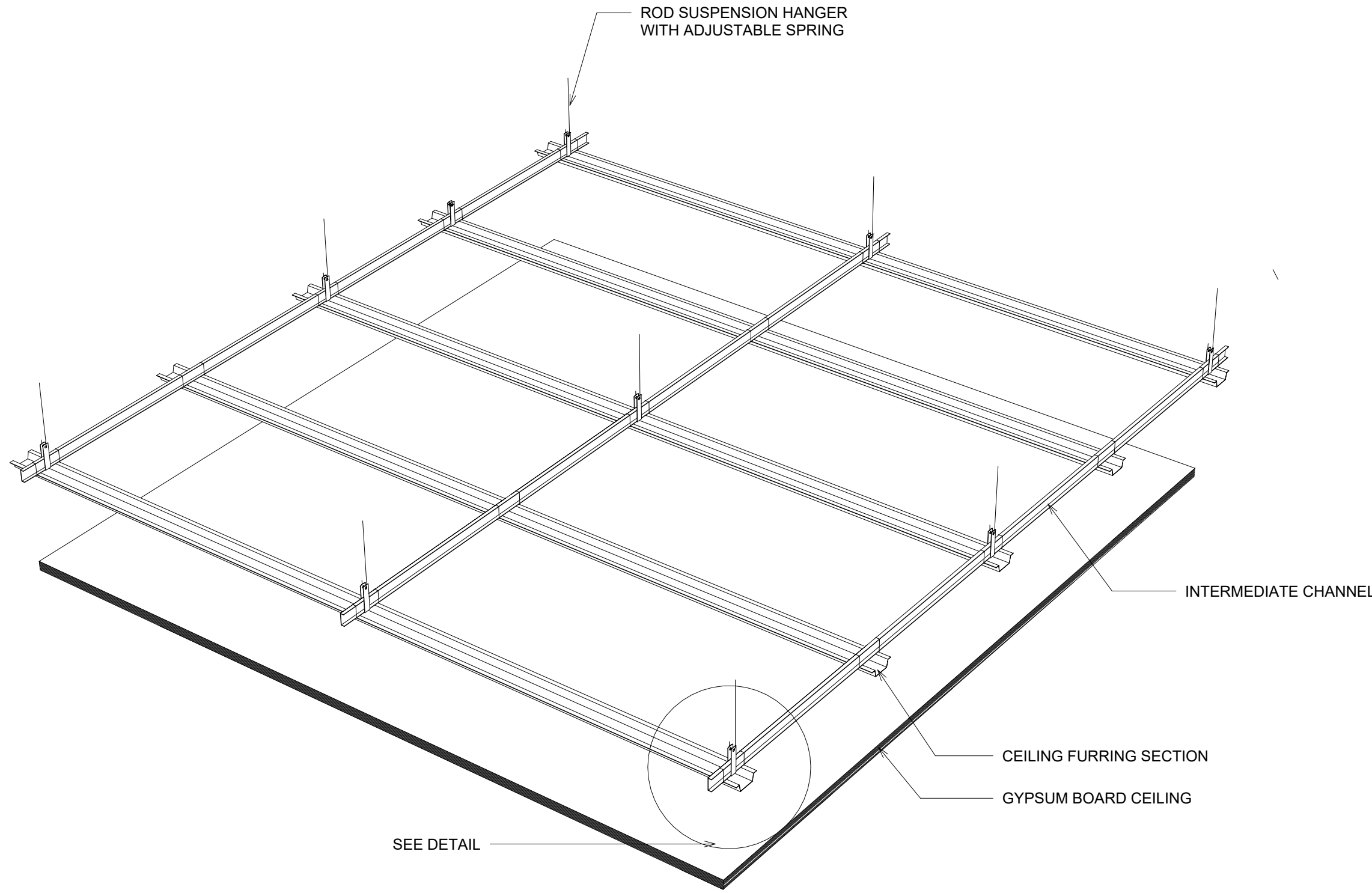
1 TYPICAL 3D VIEW - GYPSUM BOARD CEILING 1 : 100
