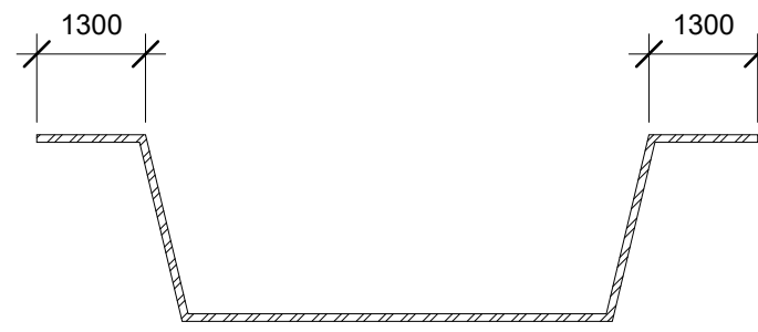
8 FURRING CHANNEL 1 : 100
