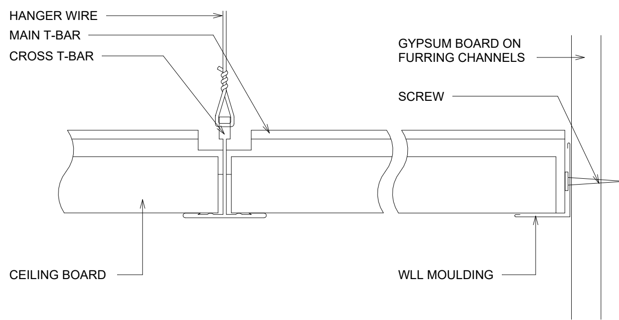
11 SECTION PERPENDICULAR TO MAIN T-BAR 1 : 100
