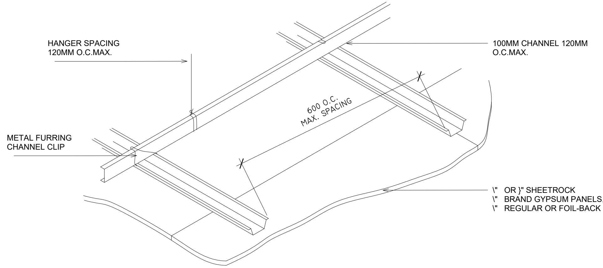
2 TYP. 3D GYPSUM STEEL FRAMED FURRING CHANNEL 1 : 5
