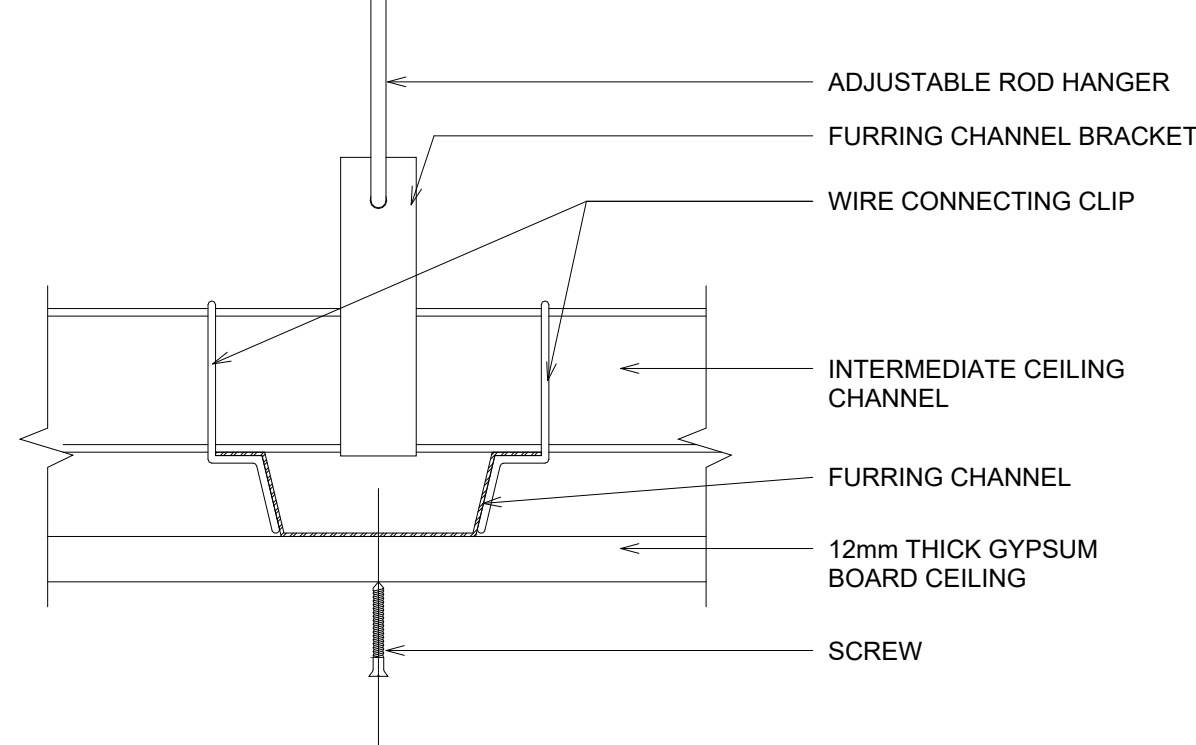
4 SECTION AT FURRING CHANNEL 1 : 100
