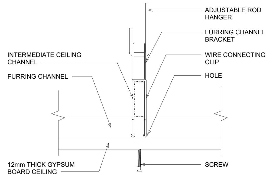
3 SECTION AT INTERMEDIATE CHANNEL 1 : 100
