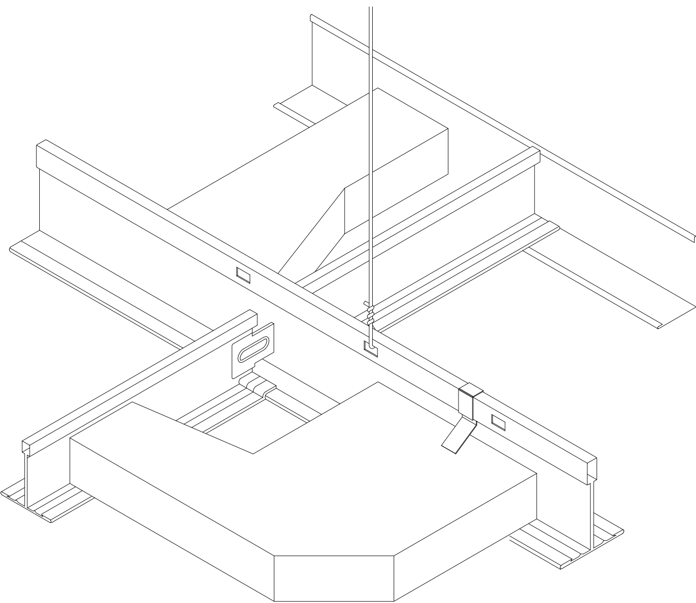
9 DETAIL OF EXPOSED T-BAR SYSTEM 1 : 100
